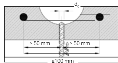
3. Make a cylindrical hole.
